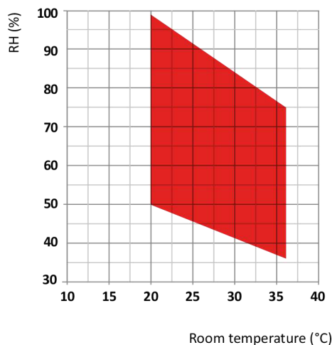
Operation limits
